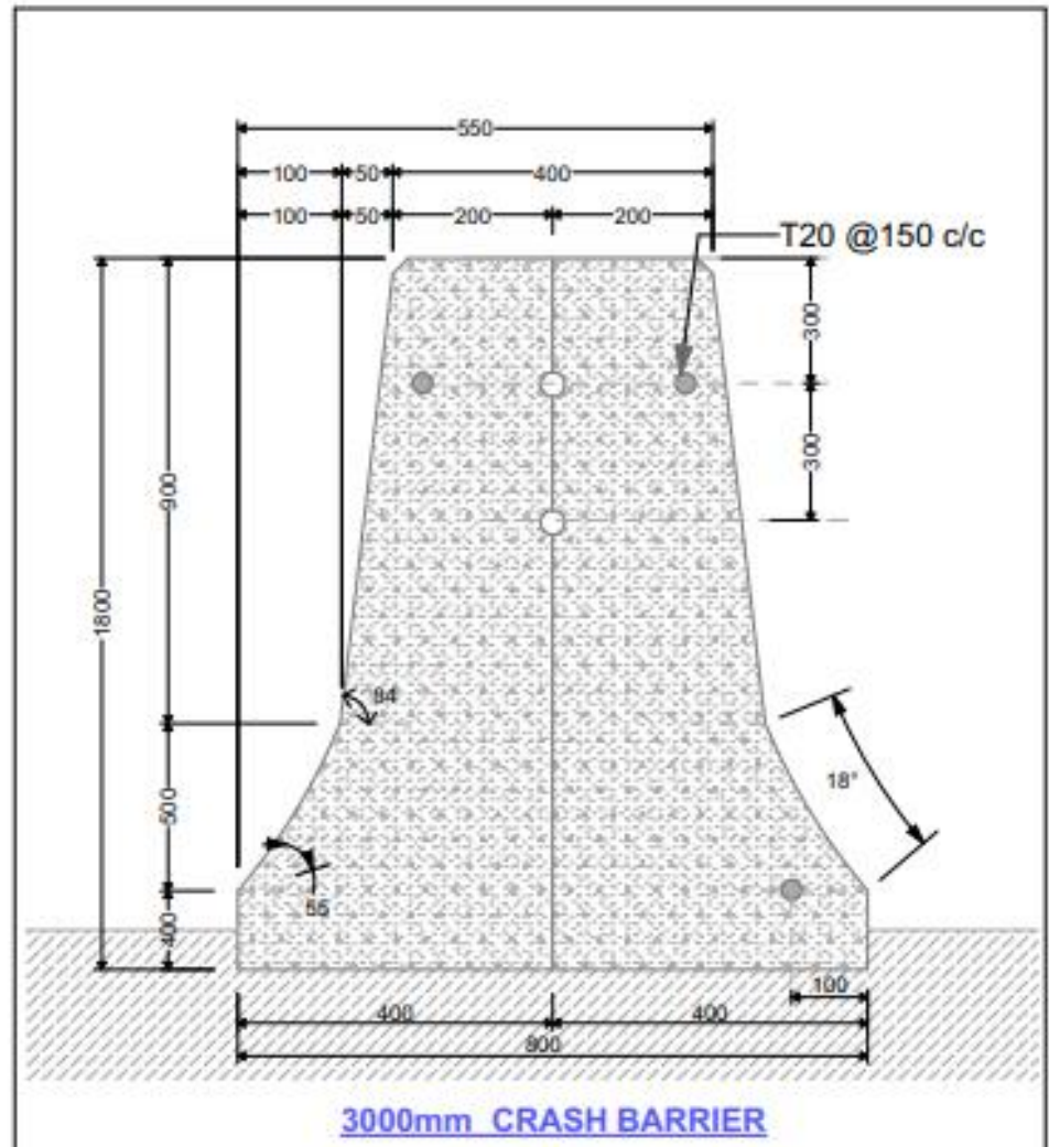
DRAWING: CROSS-SECTION OF THE REINFORCED CONCRETE CRASH BARRIER
