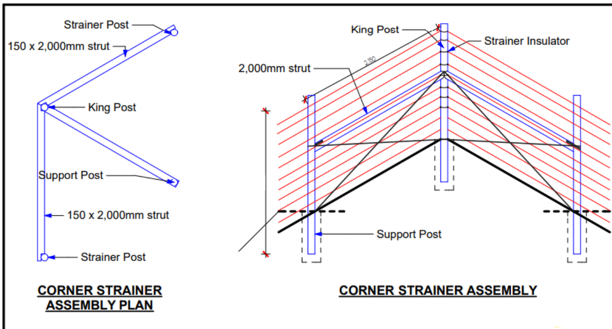
Drawing 01: SGR Game Proof Electric Fence.
